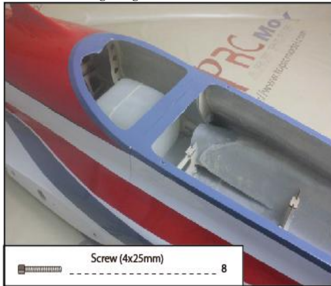
34.Fix the fuselages together with screws.
